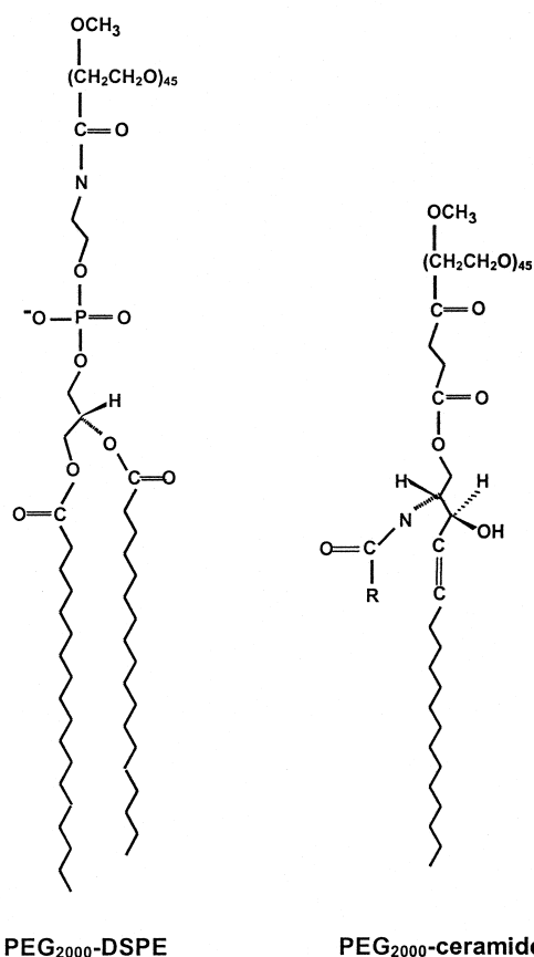
Fig. 1. Chemical structures of PEG-DSPE and PEG-ceramides. The structure for PEG 2000 -DSPE is modified from that provided by Avanti Polar Lipids and it is assumed that 45 poly(ethylene glycol) groups are used to comprise a 2000 Da PEG moiety. For the PEG-ceramides, the R group was C 7 H 15 (for the C8-ceramide), C 13 H 27 (for the C14-ceramide), C 15 H 31 (78 mol%; for the egg ceramide), C 19 H 39 (for the C20-ceramide) or C 23 H 47 (for the C24-ceramide).
