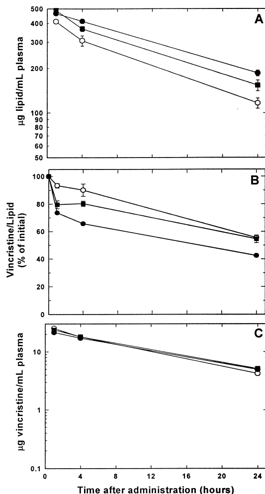
Fig. 3. Pharmacokinetic analysis of SM/chol (55:45, mol/mol) (○), SM/chol/PEG-DSPE (50:45:5, mol/mol/mol) (●) and SM/chol/PEG-CER (C16) (50:45:5) (■) formulations of vincristine. (A) Concentrations of liposomal lipid in the plasma at various times after i.v. administration. (B) Vincristine/lipid ratio (% of the administered vincristine/lipid ratio) in the plasma at various times after i.v. administration. (C) Concentrations of vincristine in the plasma at various times after i.v. administration. Data represent the mean ( \pm S.E.) of four animals.
